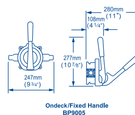
On Deck/Fixed Handle BP9005
